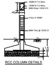
RCC COLUMN DETAILS
