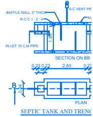
SEPTIC TANK AND TRENCH
