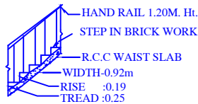
STAIR DETAIL
