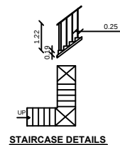
STAIRCASE DETAILS
