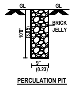
PERCOLATION PIT
