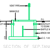
SECTION OF SEP.TANK
