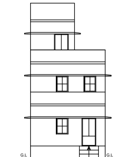
FRONT ELEVATION
