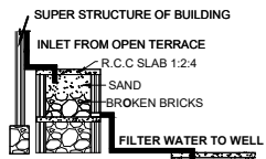
RAINWATER HARVESTING
