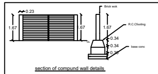
section of compound wall details
