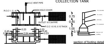
SEPTIC TANK DETAILS
