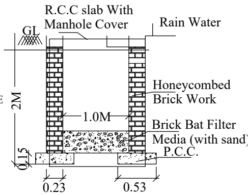
Details Of Rain Water Collection Pit (Recharge Well Method) SCALE:- (NTS)
