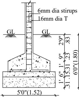
COLUMN FOUNDATION DETAIL SCALE (NTS)
