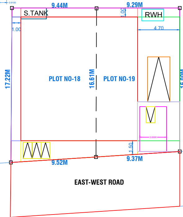
SITE PLAN(1:100)
