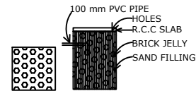
PLAN & SECTION OF RAINWATER COLLECTION TANK
