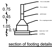
section of footing details
