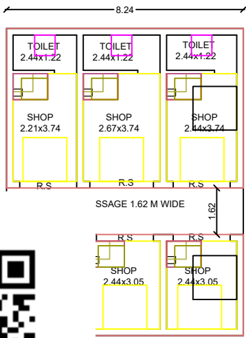
ST FLOOR PLAN
