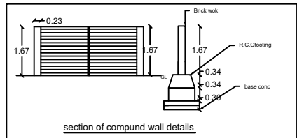
section of compound wall details
