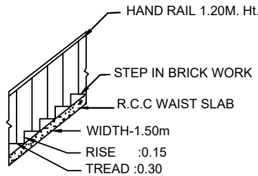
STAIR DETAIL
