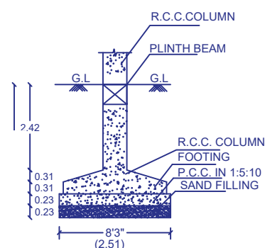
FOUNDATION DETAIL (DETAIL - B)
