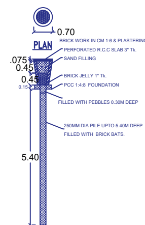
PERCOLATION PIT
