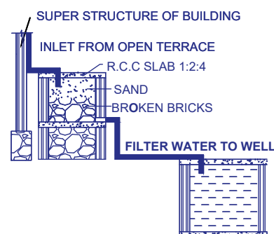
RAINWATER HARVESTING
