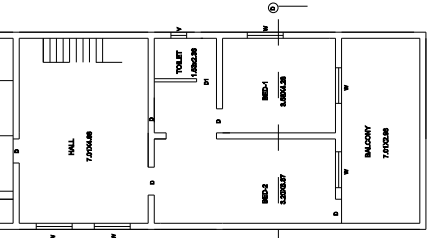
F. FLOOR PLAN
