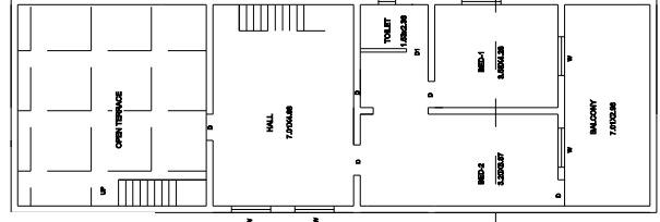
F. FLOOR PLAN
