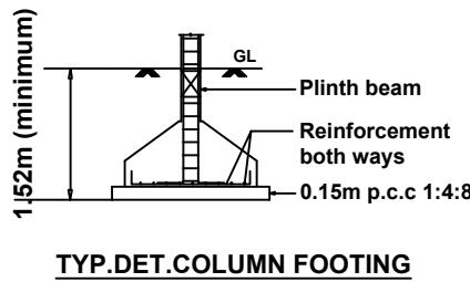
TYP.DET.COLUMN FOOTING
