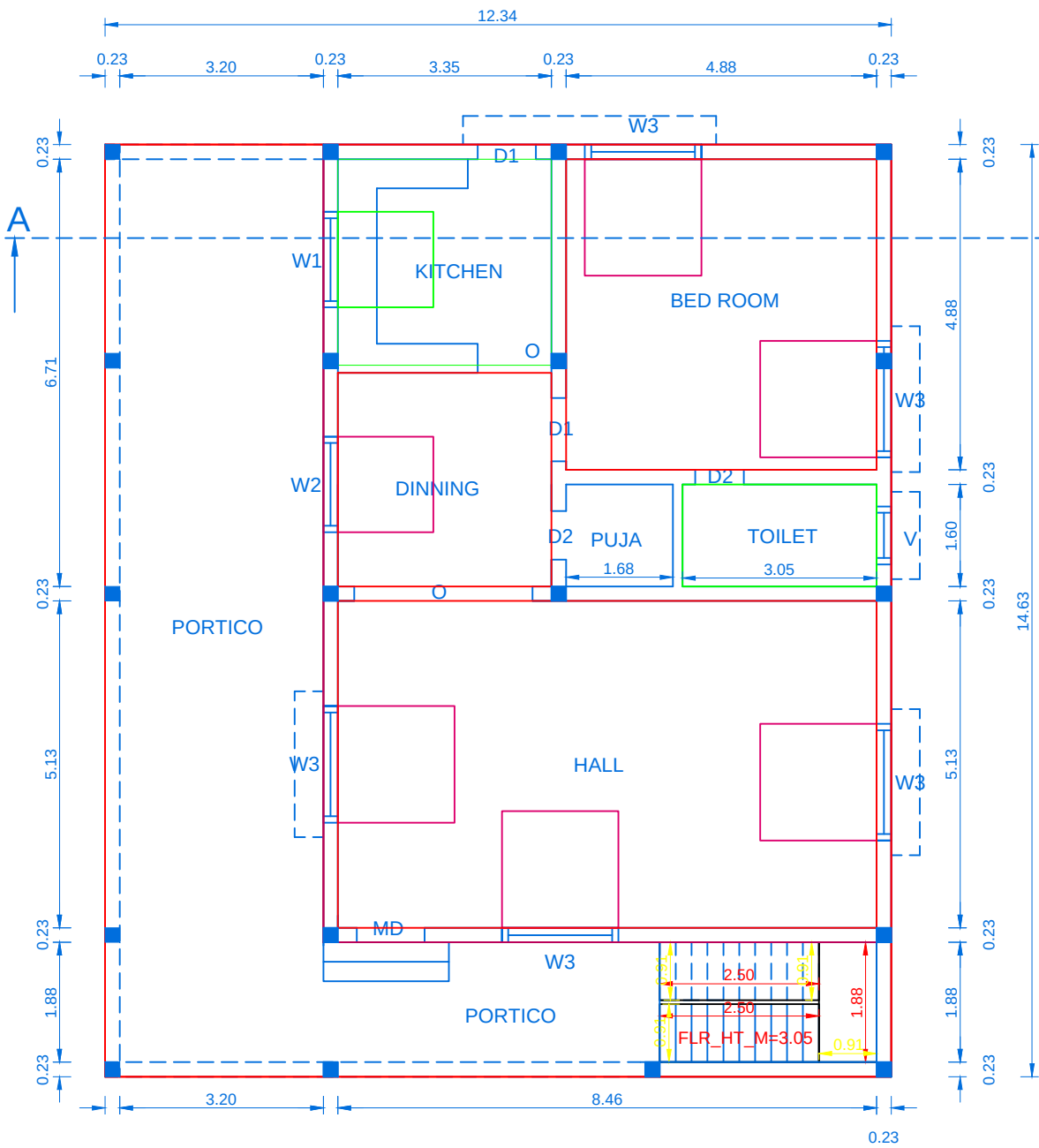
JND FLOOR PLAN
