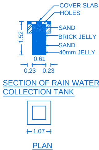
PLAN
