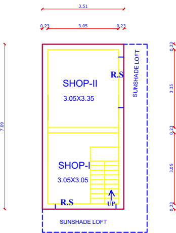
PROPOSED FIRST FLOOR PLAN SHOPS-I& II
