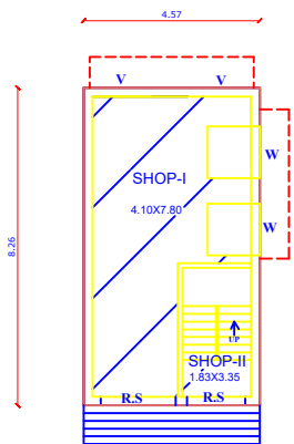
EXG- GROUND FLOOR PLAN SHOPS(I&II) DOOR NO:117 &117A
