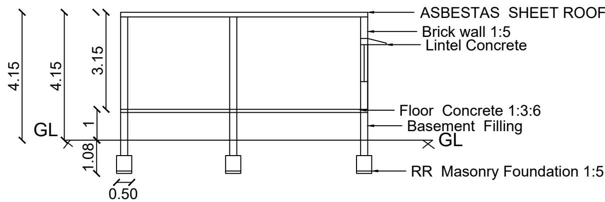
SECTION A-A VIEW
