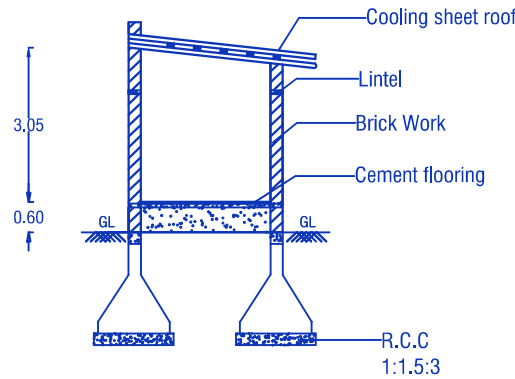
CROSS SECTION ON 'AB'
