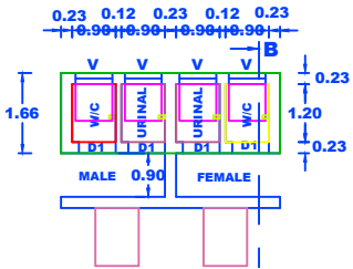
PRO.GROUND FLOOR PLAN
