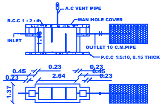
SEPTIC TANK & TRENCH
