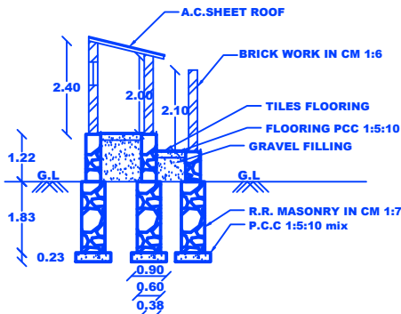
SECTION ON 'BB'
