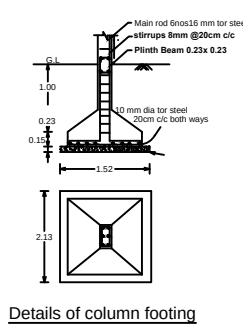
Details of column footing
