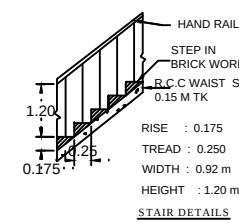
STAIR DETAILS
