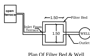
Plan Of Filter Bed & Well
