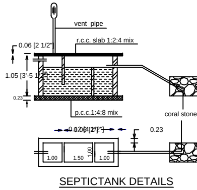
SEPTICTANK DETAILS
