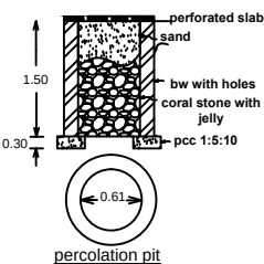
percolation pit
