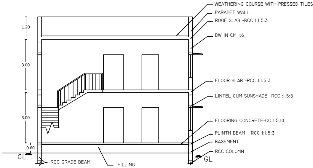
SECTION- XX
