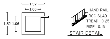
STAIR DETAIL
