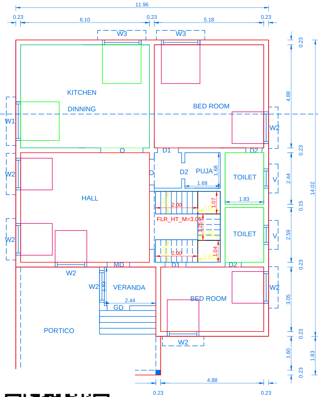
ID FLOOR PLAN
