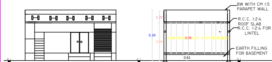
FRONT ELEVATION
