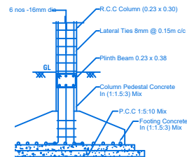
COLUMN FOOTING DETAILS
