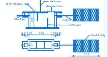
SEPTIC TANK & TRENCH
