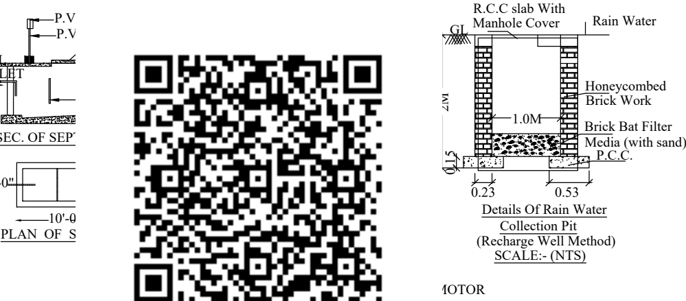
DETAILS OF RAIN WATER COLLECTION PIT (RECHARGE WELL METHOD) SCALE:- (NTS)
