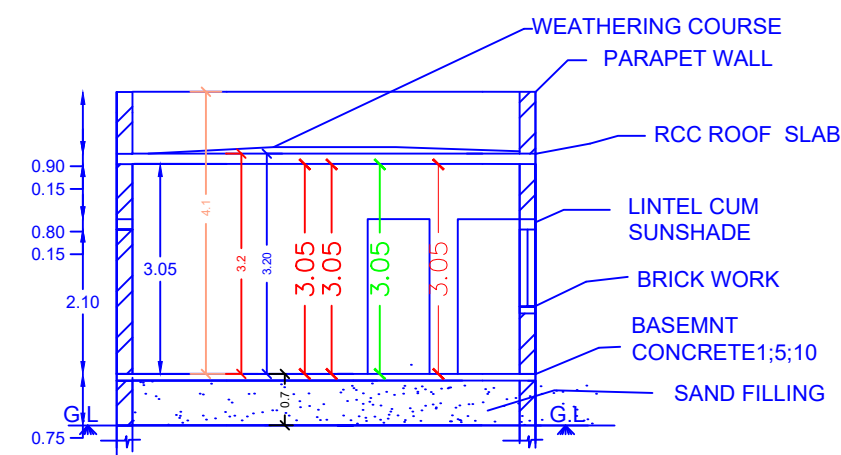
SECTION AB
