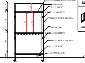
SECTION ON AB&amp;CD
