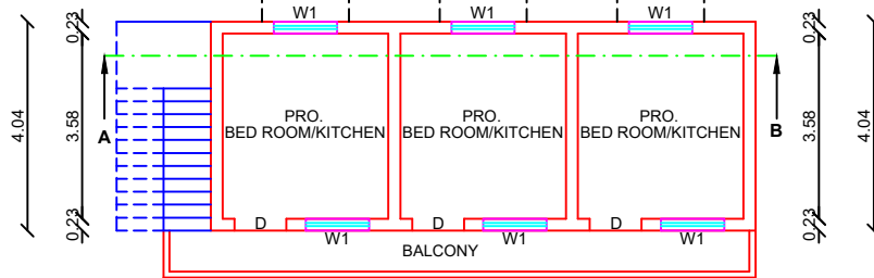
PRO. FIRST FLOOR PLAN
