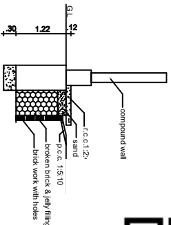
PLINTH BOUNDARY PERCOLATION PIT
