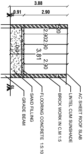
SECTION-AB
