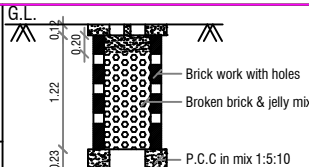
PERCOLATION PIT FOR 30 Sq. m.
