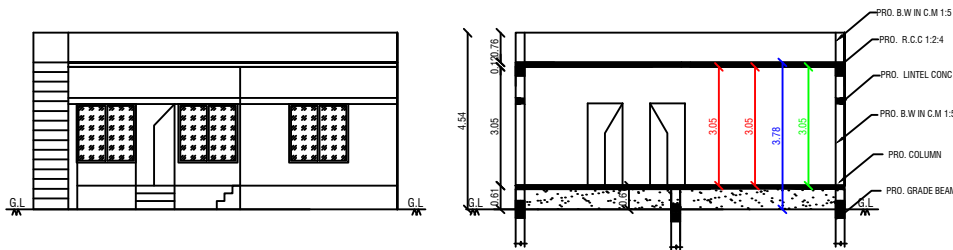
FRONT ELEVATION
