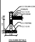
Column Details
