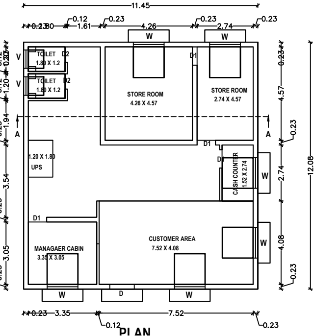
PLAN
