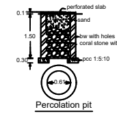
Percolation pit
