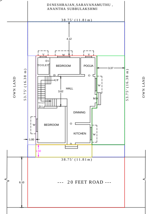
SITE PLAN
