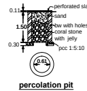
percolation pit
