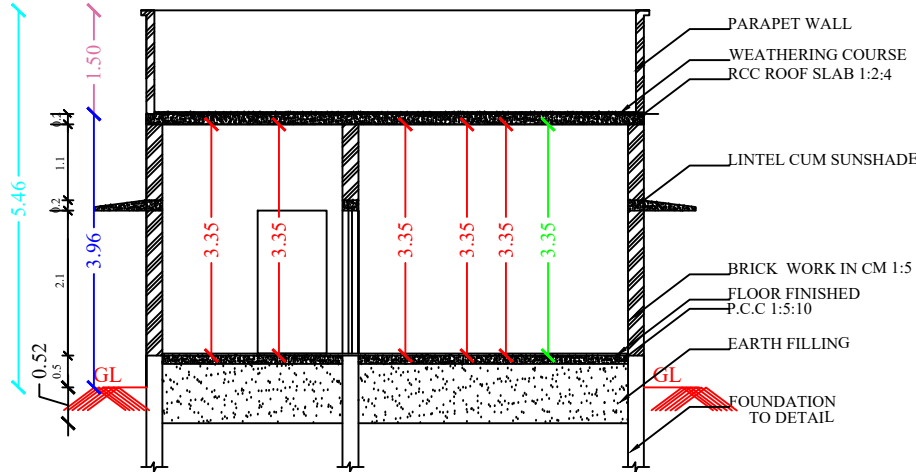
SECTION "A-B"
