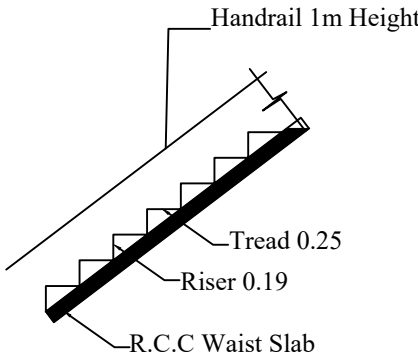
STAIR DETAILS
