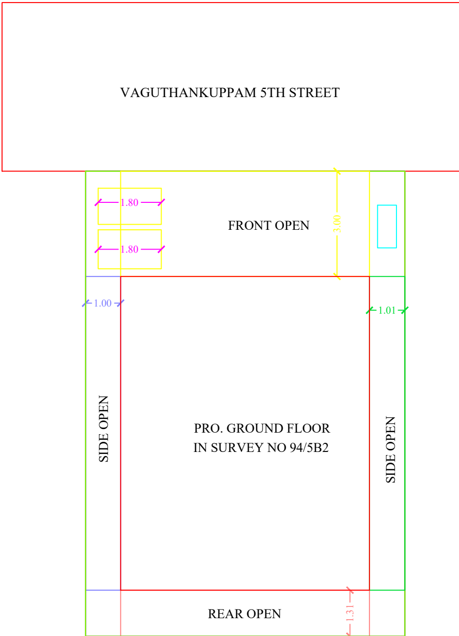
SITE PLAN
