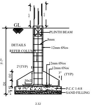
FOUNDATION DETAILS
