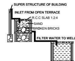
RAINWATER HARVESTING
