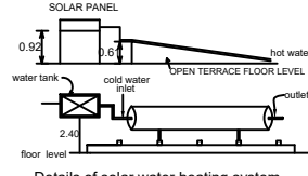
Details of solar water heating system
