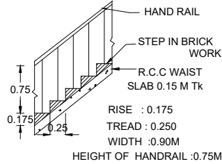
STAIR DETAILS
