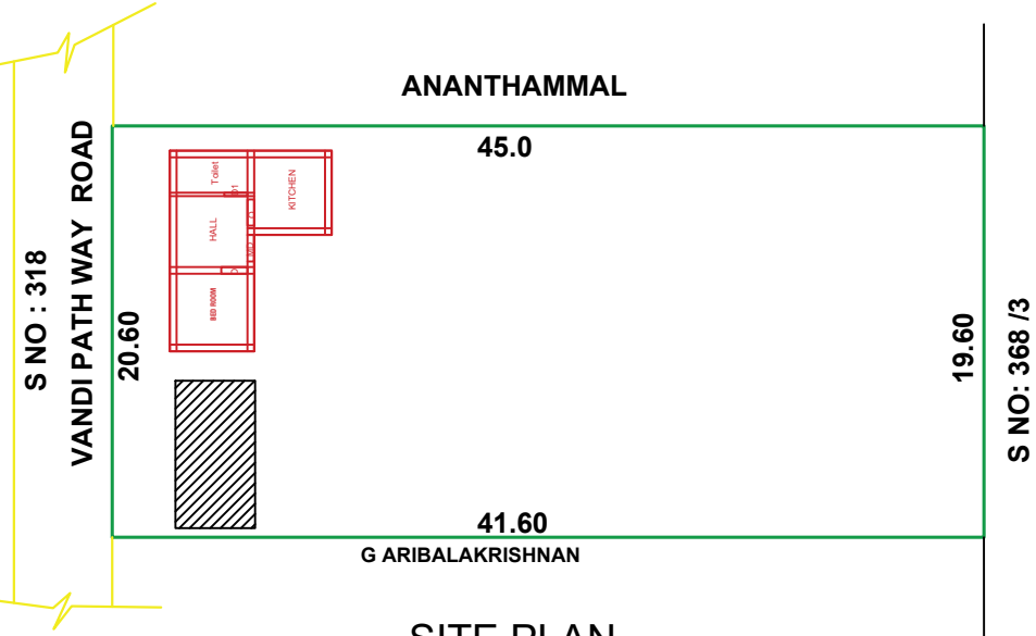
SITE PLAN
