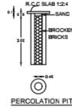
PERCOLATION PIT
