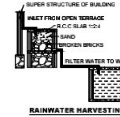
RAINWATER HARVESTING
