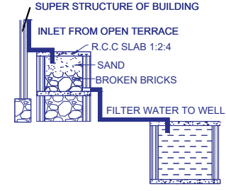
RAINWATER HARVESTING
