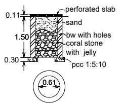
percolation pit
