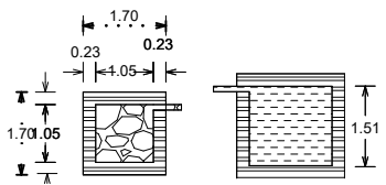
DETAILS OF FILTER BED & WELL
