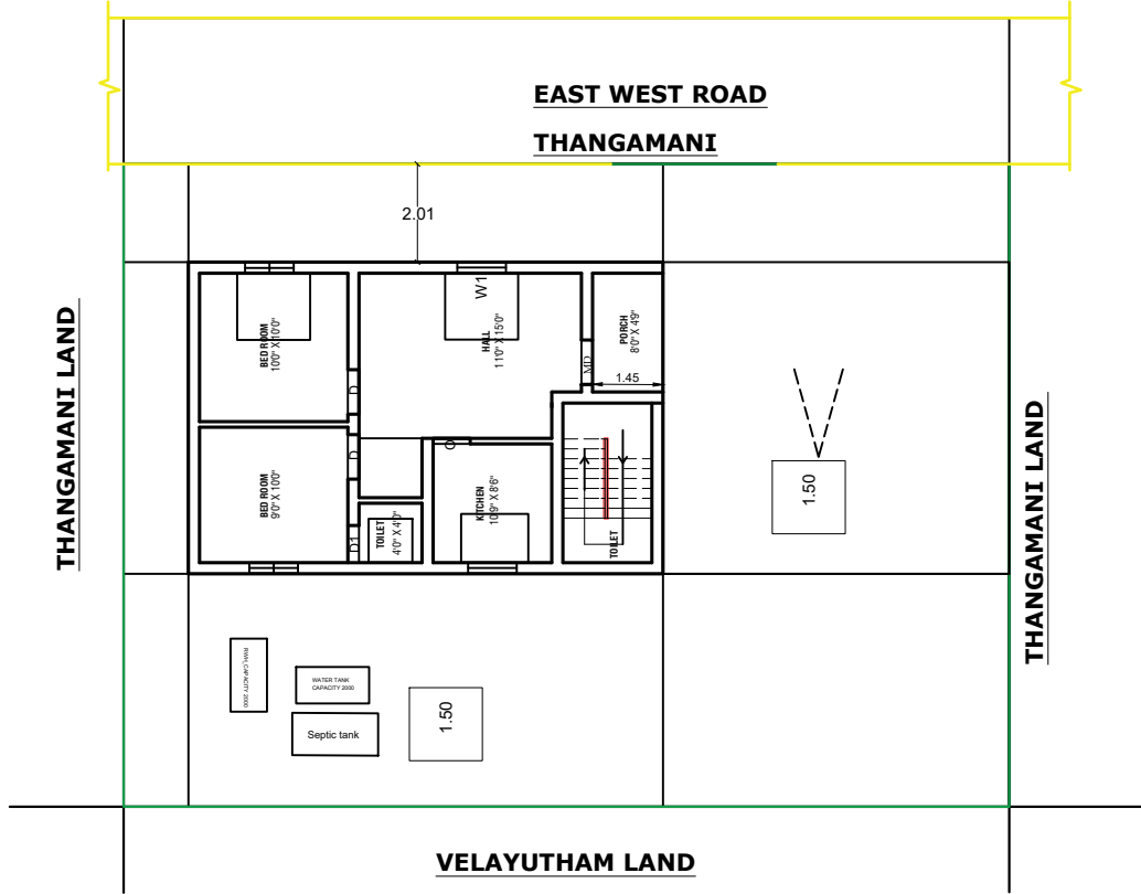
SITE PLAN
