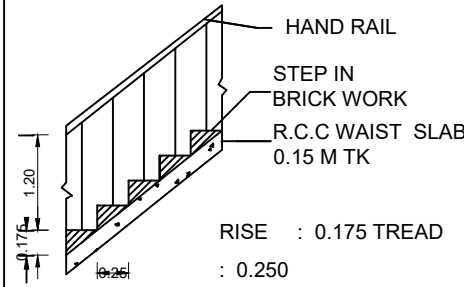
STAIR DETAILS
