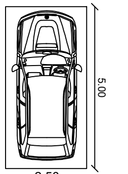
CAR POCKET DETAILS
