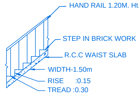
STAIR DETAIL
