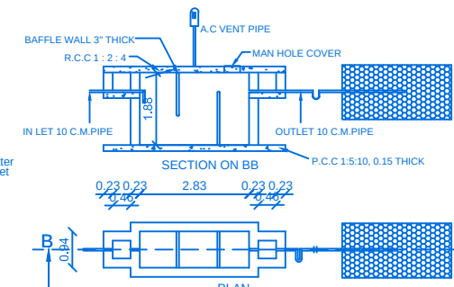
SECTION ON BB
