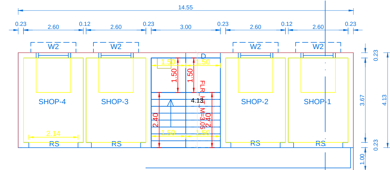
OUND FLOOR PLAN
