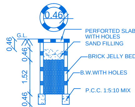
PERCOLATION PIT
