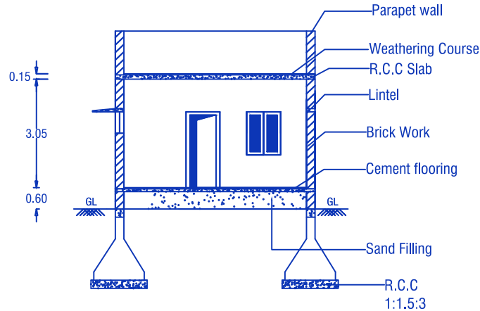
CROSS SECTION ON 'AB'
