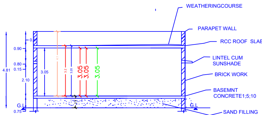
SECTION AB
