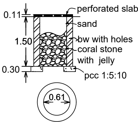
PERCOLATION PIT
