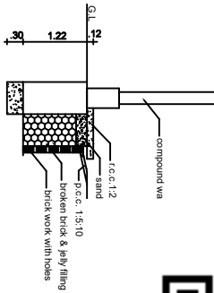
PLINTH BOUNDARY PERCOLATION PIT
