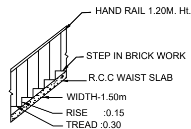
STAIR DETAIL
