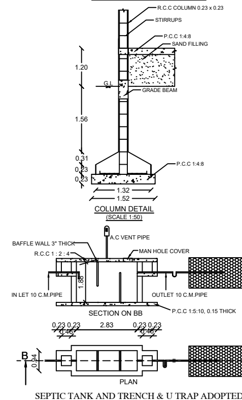
SEPTIC TANK AND TRENCH & U TRAP ADOPTED
