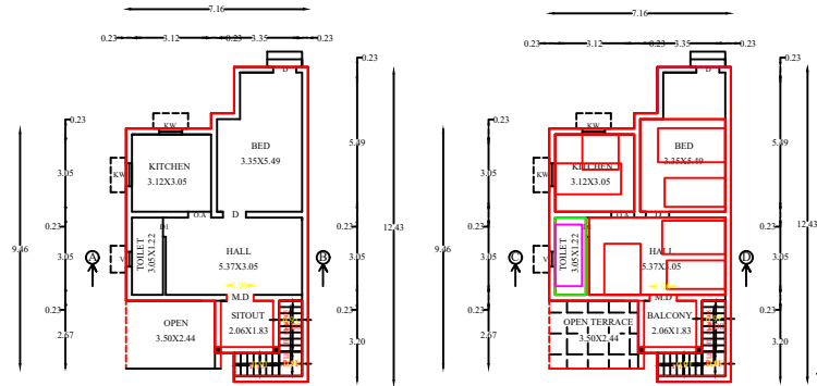
EXG.GROUND FLOOR PLAN
