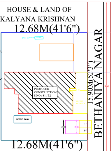
SITE PLAN
