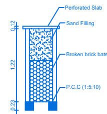
RAIN WATER COLLECTION WELL
