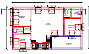
PRO.GROUND FLOOR PLAN
