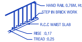
STAIR CASE DETAIL
