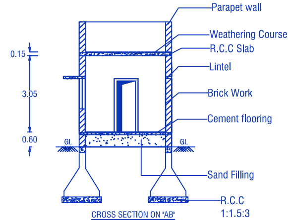
CROSS SECTION ON 'AB'
