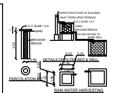
RAIN WATER HARVESTING
