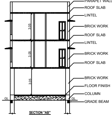
SECTION "AB"
