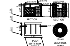
PLAN LEACH WELL DETAIL
